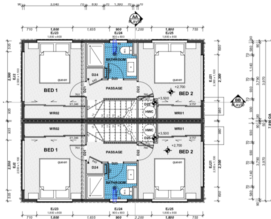
TOTAL SECOND FLOOR AREA: 36 SQM
